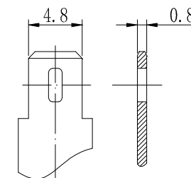
Terminal T1
